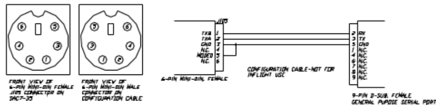
Figure 4-1 6 Pin Din to Serial Interconnect
