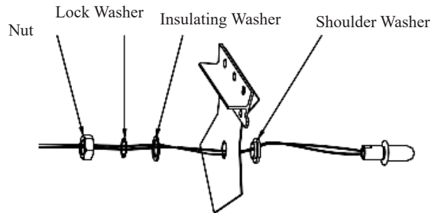
Figure 3-4 STP 78 OAT Probe Mounting
