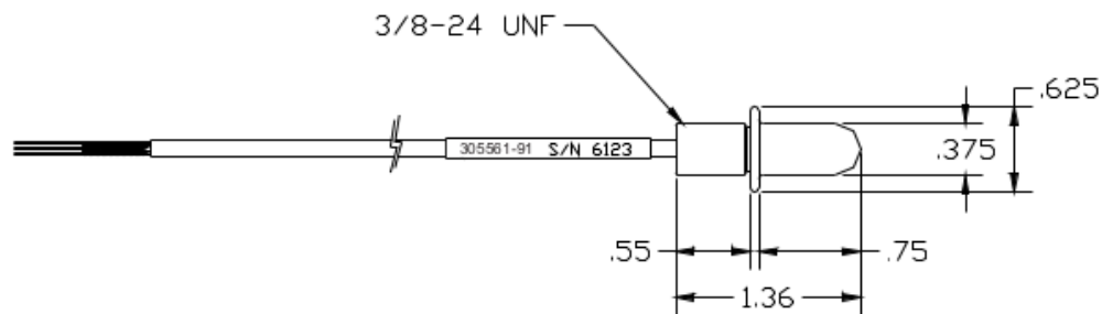
Figure 3-3 STP 78 OAT Probe Dimensions
