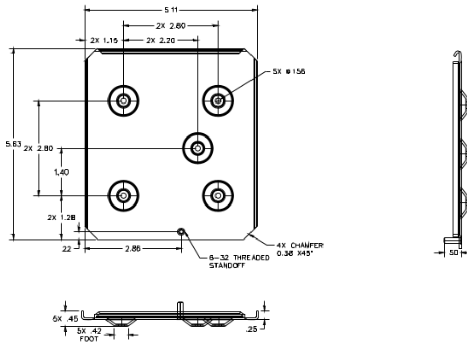
Figure 3-1 Mounting Tray Dimensions
