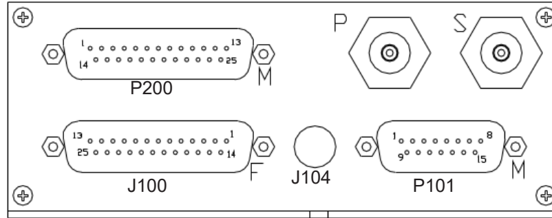
Figure 3-9 Front Panel Connector Location
