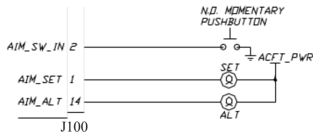
Figure 3-6 AIM Interconnect
