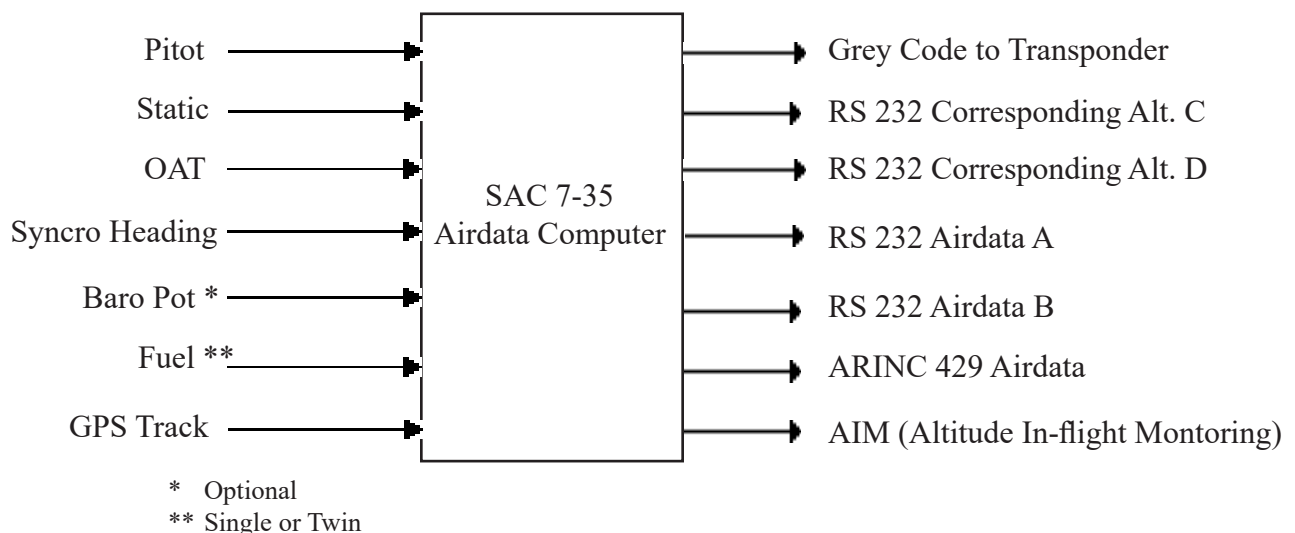
Figure 1-1 System Configuration
