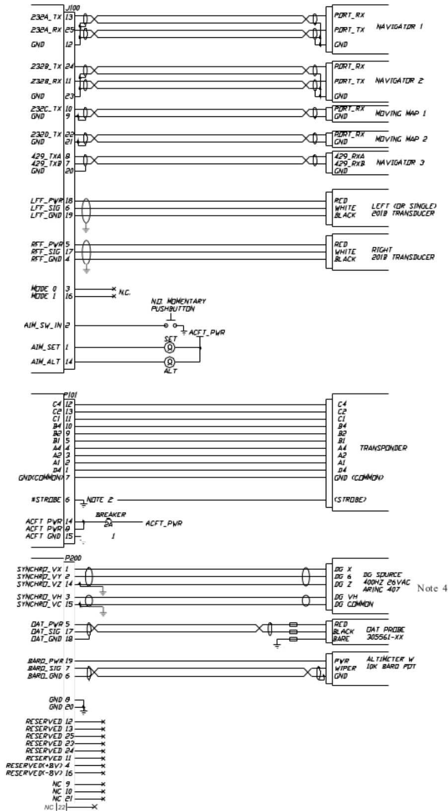
Figure 3-8 SAC 7-35 Interconnect Wiring Diagram
