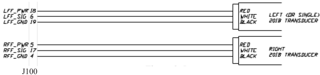
Figure 3-5 Fuel Flow Interconnect
